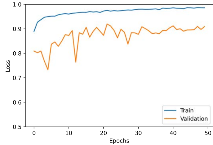
Overfitting
