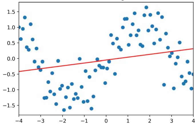
Underfitting
