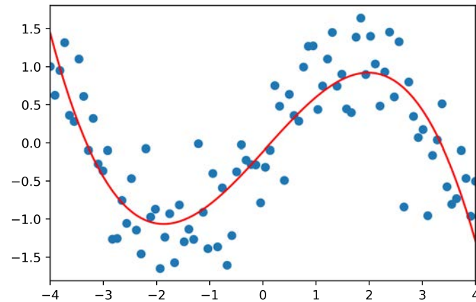
Good Fit
