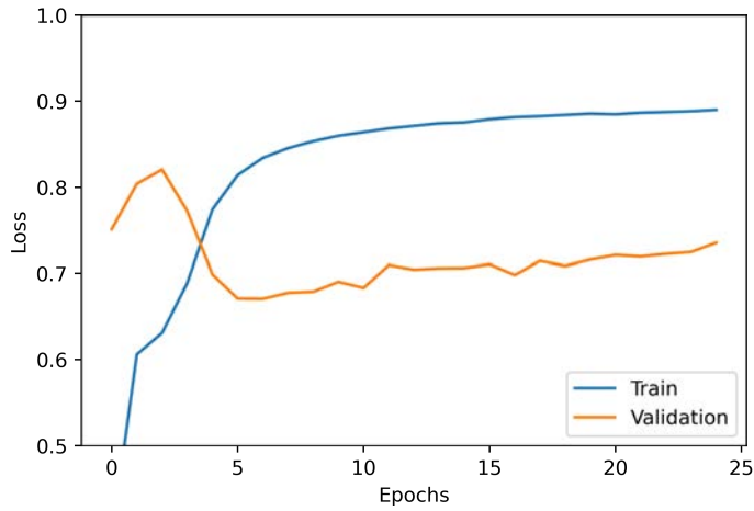
Underfitting
