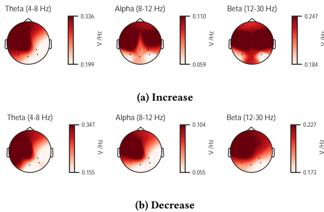
Figure 2: Topographic maps for the increase and decrease variations of secondary task difficulty for the EEG oscillations of interest. View is top looking down with nose at top.
